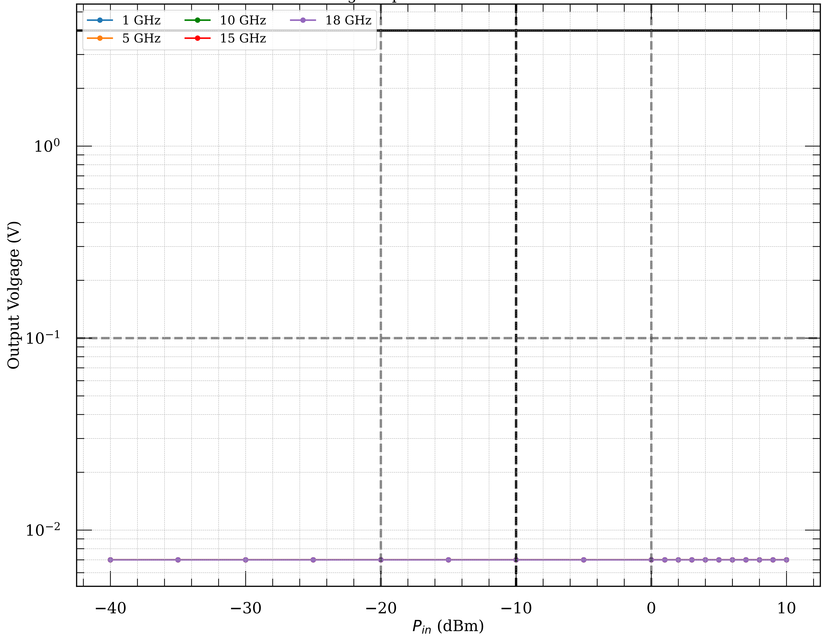
Measured voltage-to-power curve of detector module064
